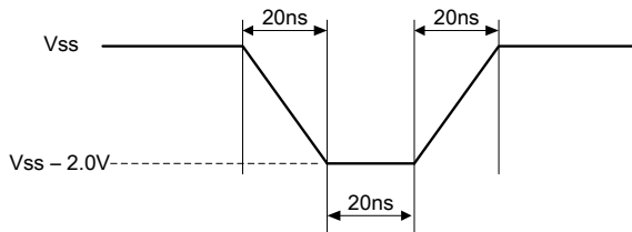
Figure 77 Maximum Negative Overshoot Waveform
