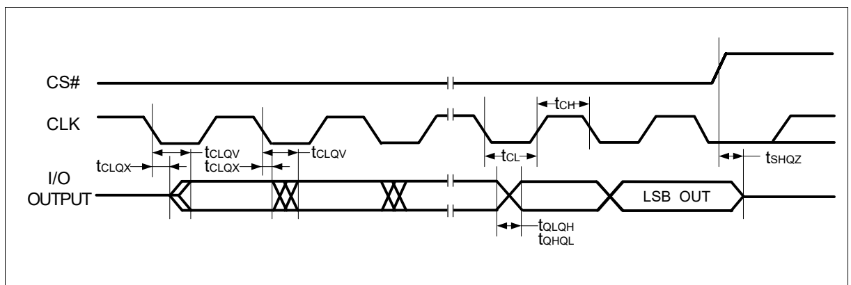
Figure 81 Serial Output Timing
