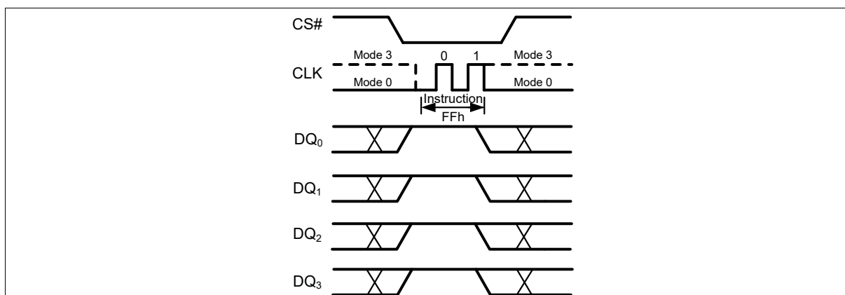
Figure 66 Disable QPI Instruction (QPI Mode only)
