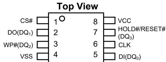
Figure 1 FM25LQ128I3 pin assignments, 8-pin SOP(208mil)
