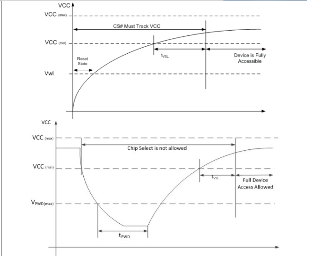
Figure 79 Power-up Timing & Power Up/Down and Voltage Drop
