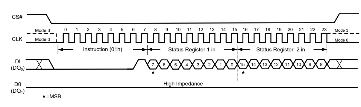
Figure 19 Write Status Register-1/2 Instruction (backward compatible, SPI Mode)
