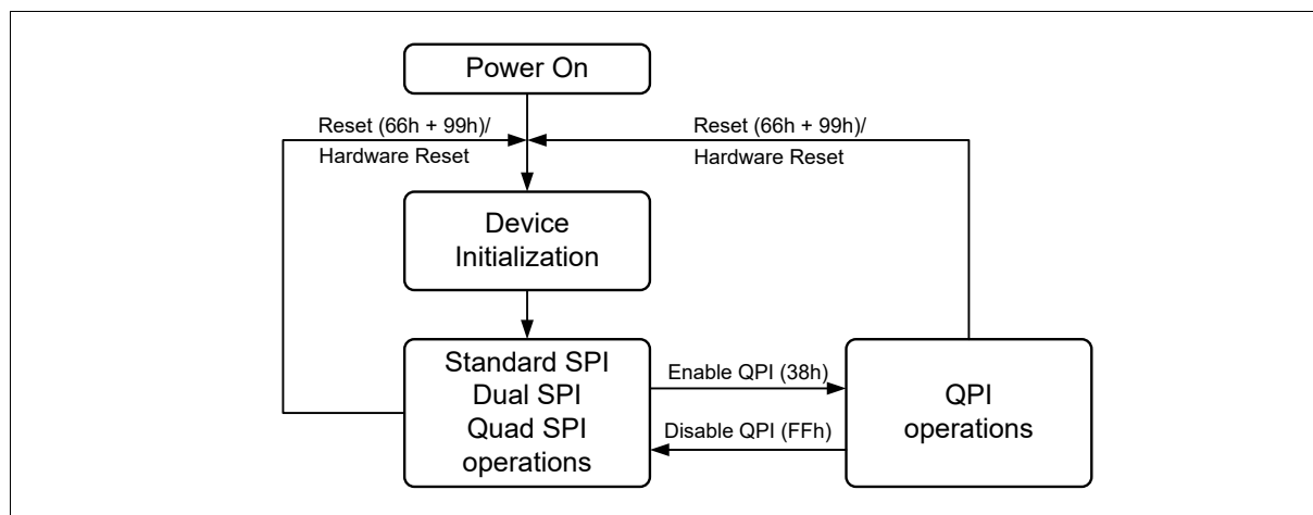
Figure 5 FM25LQ128I3 Serial Flash Memory Operation Diagram
