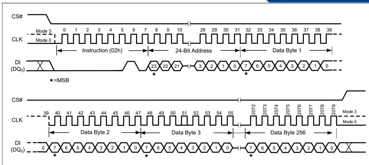
Figure 32 Page Program Instruction (SPI Mode)
