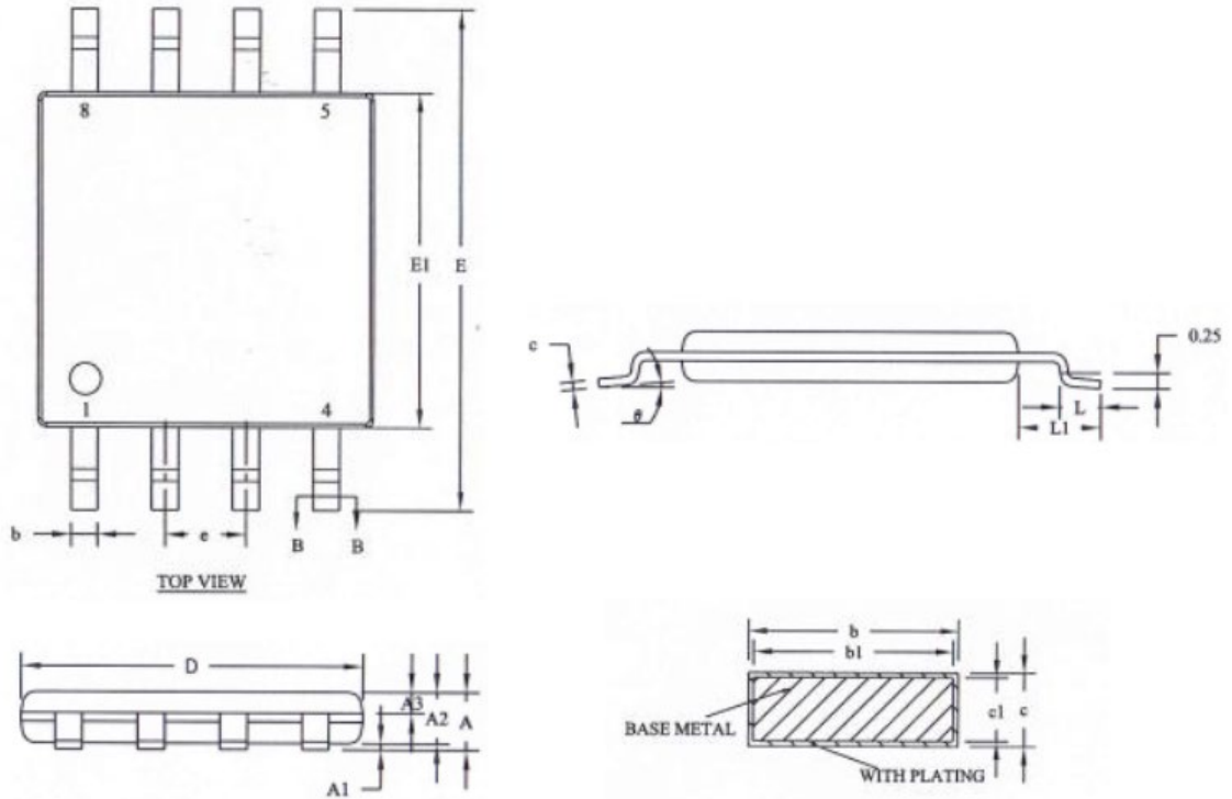
VSOP8 (208mil)
