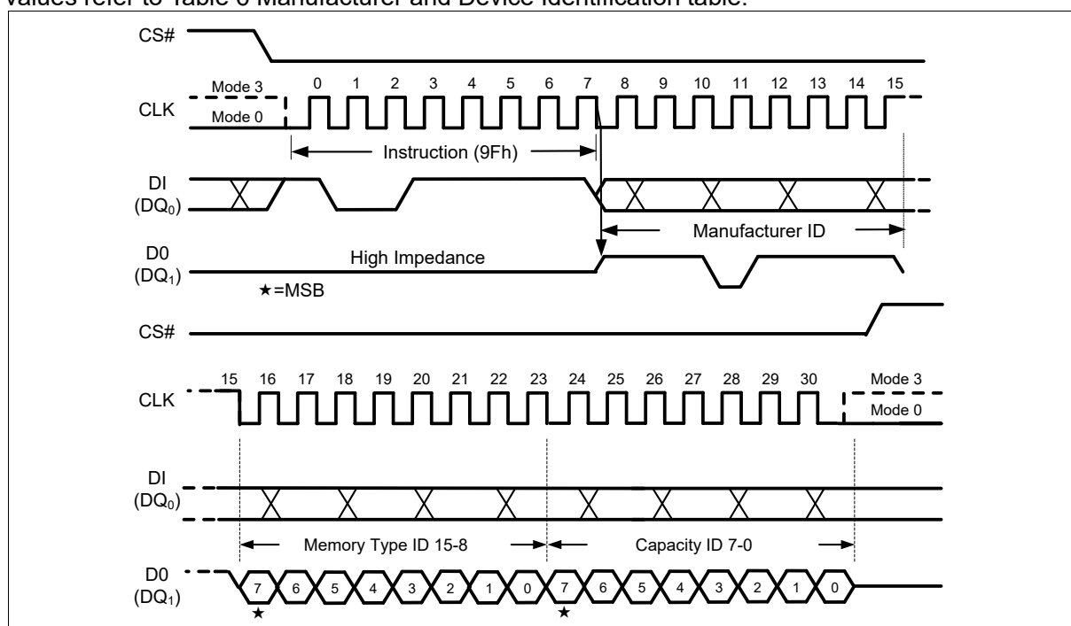
Figure 57 Read JEDEC ID Instruction (SPI Mode)
