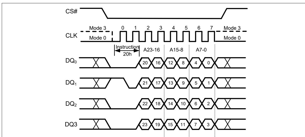
Figure 36 Sector Erase Instruction (QPI Mode)
