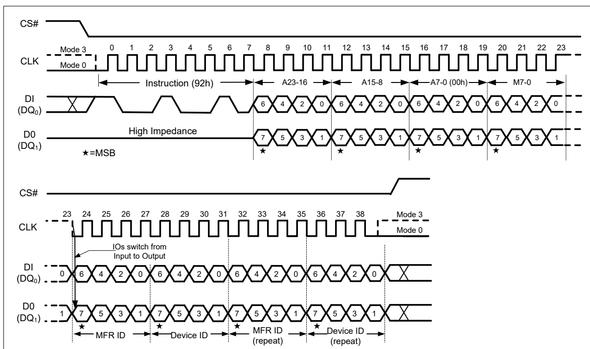
Figure 54 Read Manufacturer / Device ID Dual I/O Instruction (SPI Mode only)
