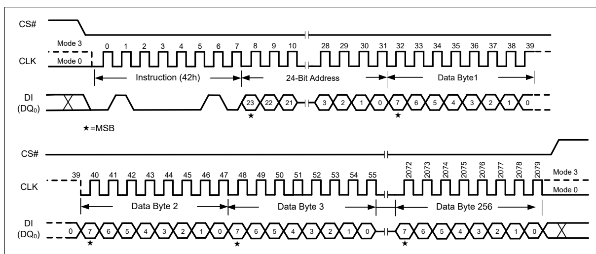
Figure 61 Program Security Sector Instruction (SPI Mode only)
