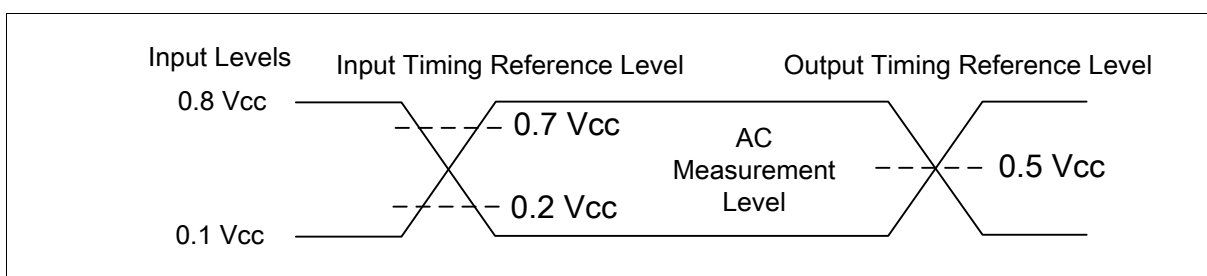
Figure 80 AC Measurement I/O Waveform
