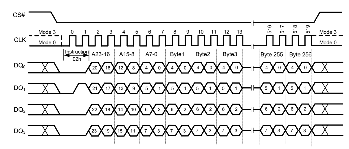
Figure 33 Page Program Instruction (QPI Mode)
