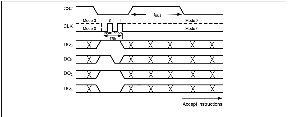
Figure 43 Erase/Program Suspend Instruction (QPI Mode)
