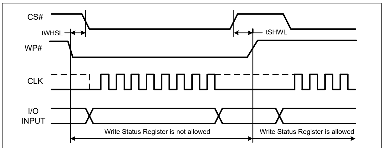
Figure 84 WP# Timing
