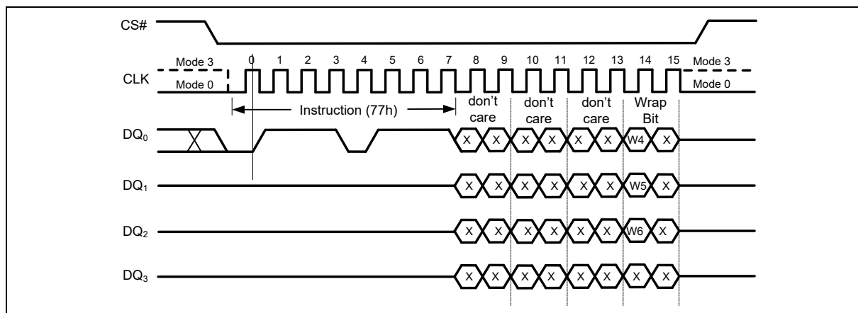
Figure 31 Set Burst with Wrap Instruction for SPI Mode
