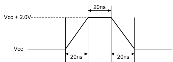
Figure 78 Maximum Positive Overshoot Waveform
