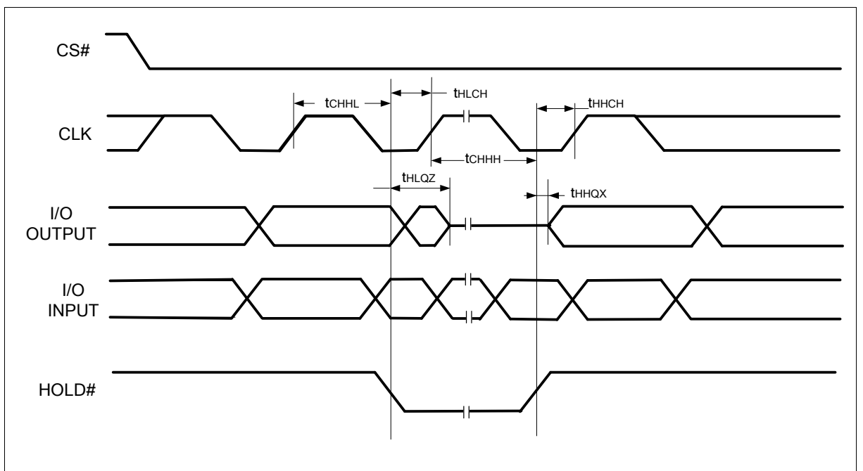
Figure 83 Hold Timing
