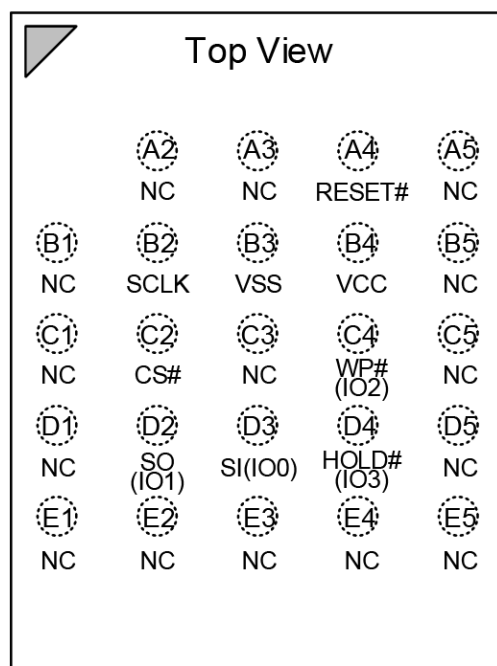
24-BALL TFBGA (5x5 ball array)
